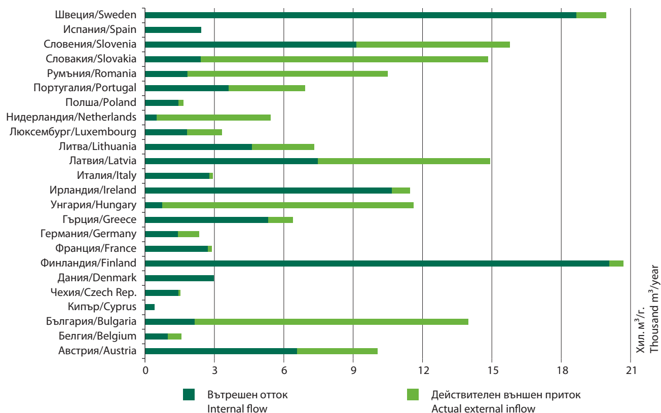
Figure 2.1. Fresh water resources per capita for some European countries
