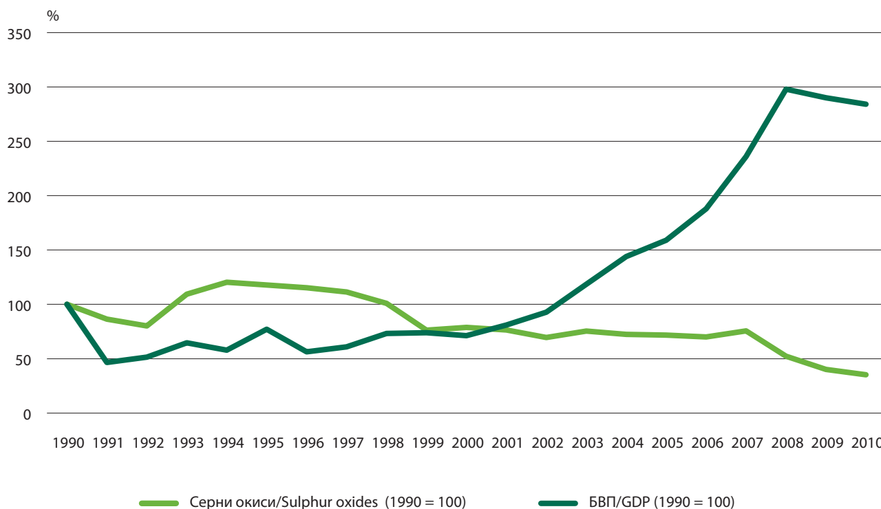
Figure 1.1. Emissions of Sulphur oxides and GDP (1990 = 100)
