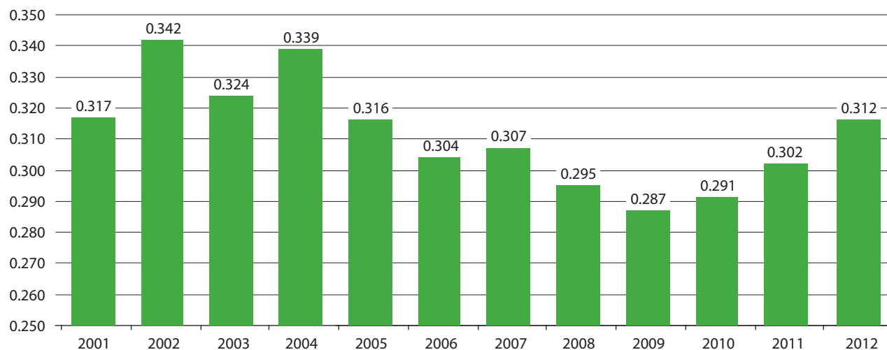
Figure 1.3. Gini coefficient
