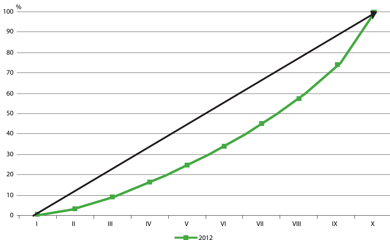
Figure 1.4. Lorenz Curve 1
